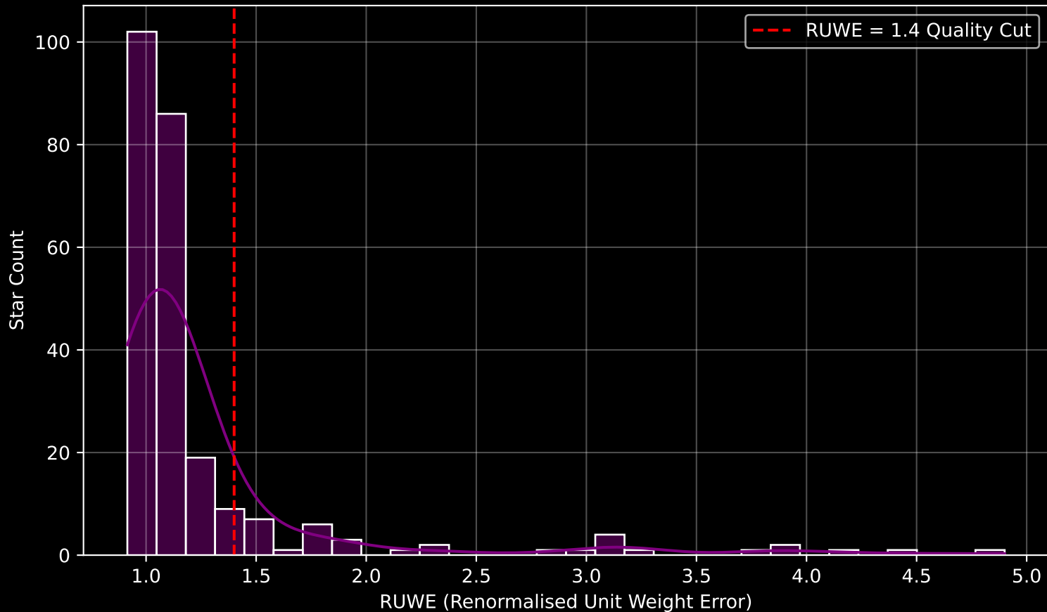
GALAH DR4 Field [2562] RUWE Distribution (n= 249)
