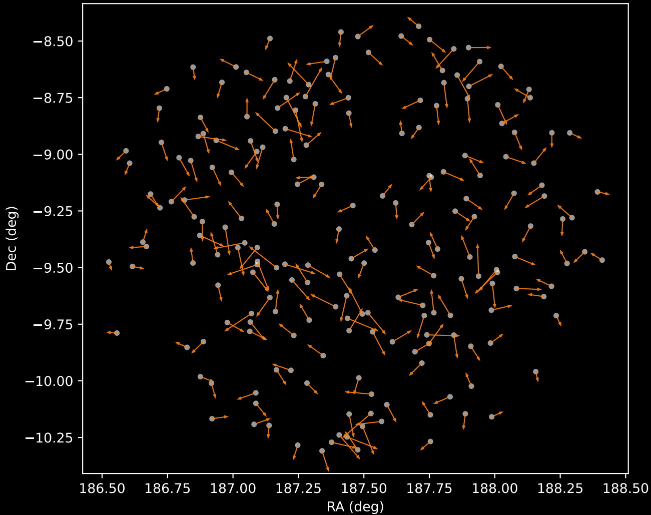
GALAH DR4 Cluster 2 Proper Motion Vectors (n=203)
