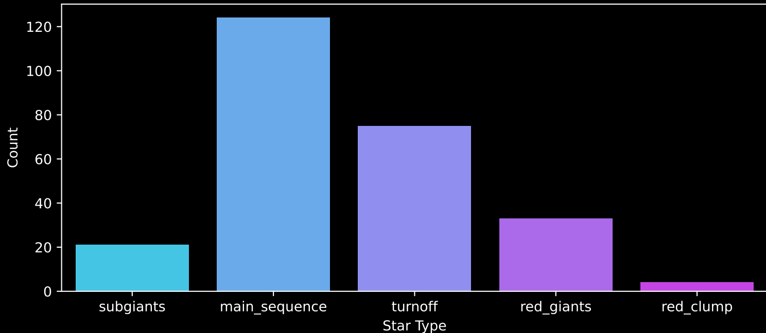
GALAH DR4 Field: [2562] Count plot of Star Type
