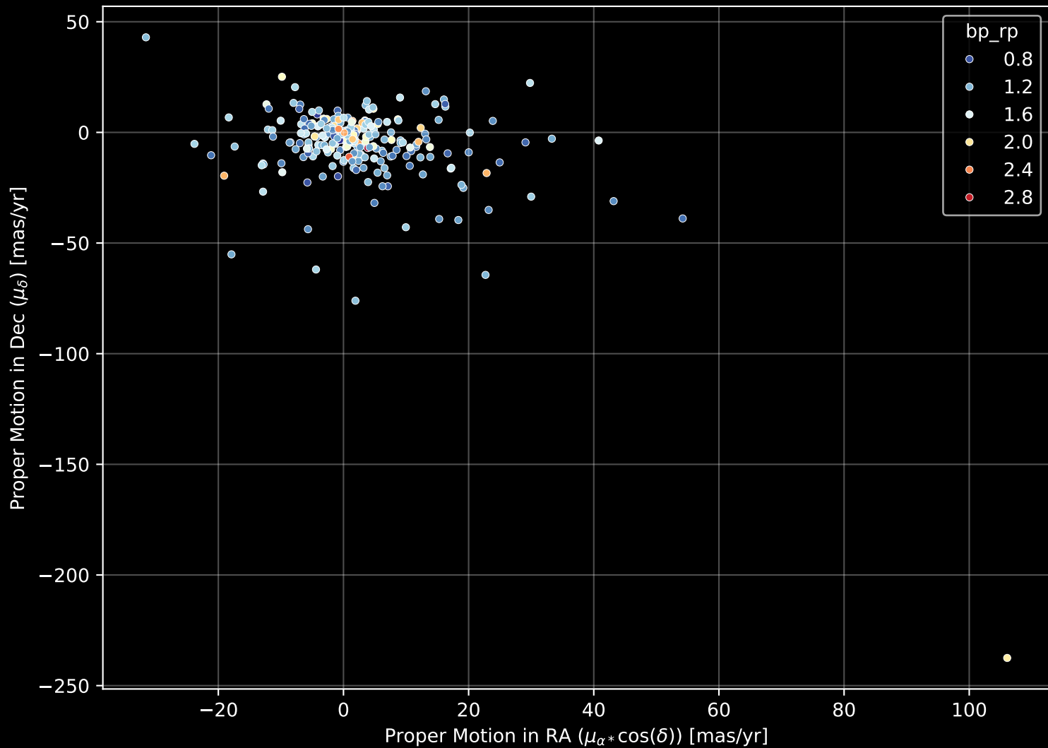
GALAH DR4 Field: [2562] Proper Motion Diagram (n= 257)
